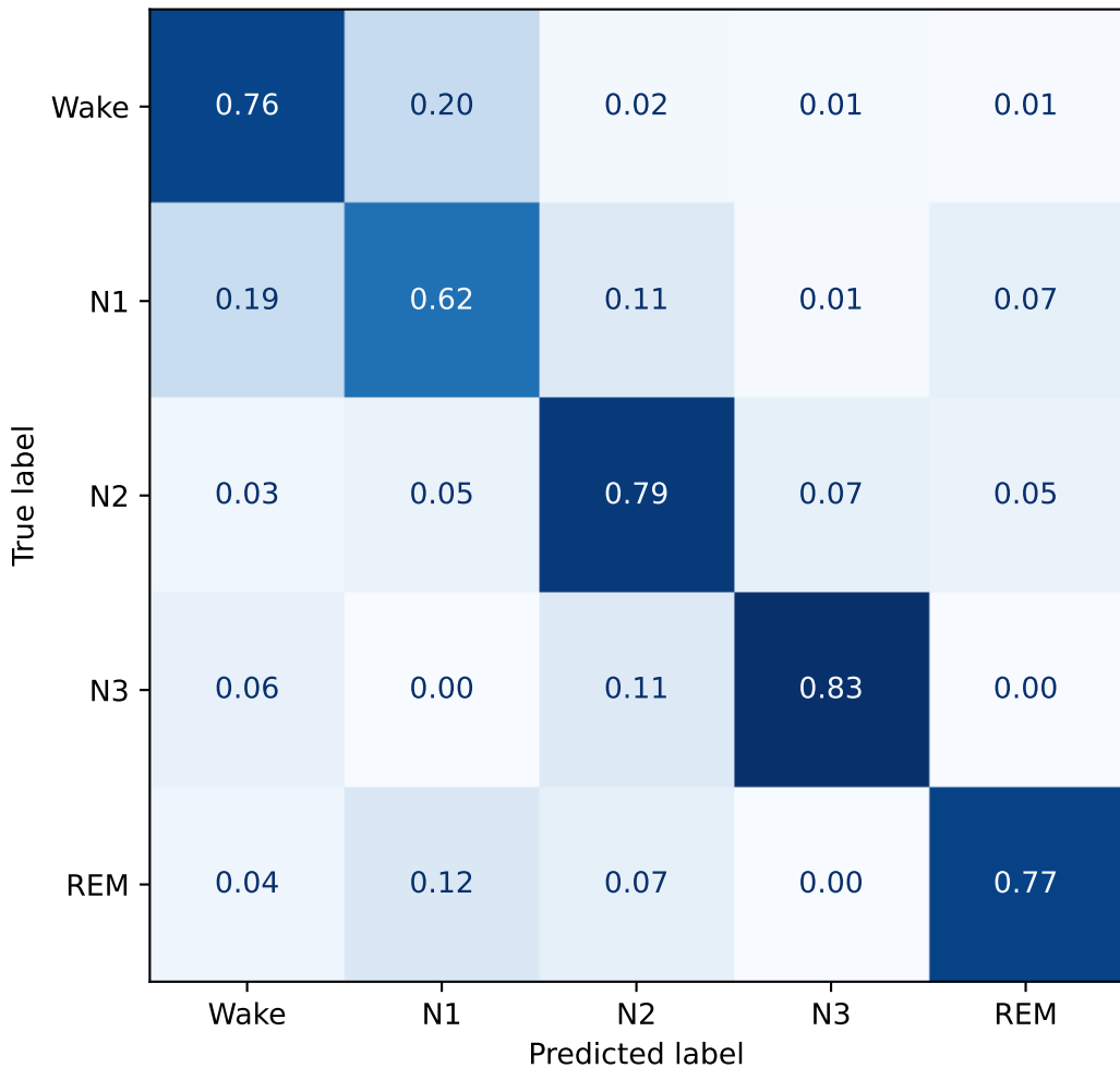
Normalised confusion matrix, test subjects 15-19
